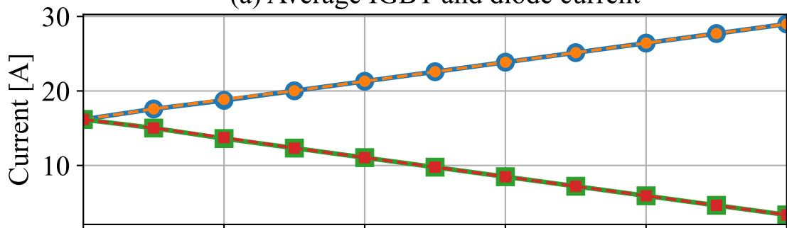
(a) Average IGBT and diode current
