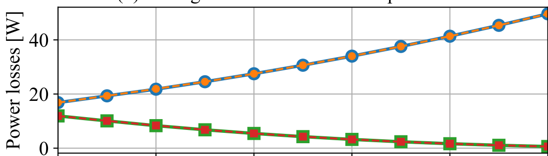
(b) Average IGBT and diode total power losses
